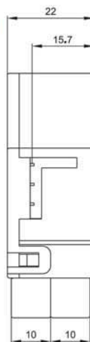
Double coil
