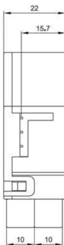
Single coil
